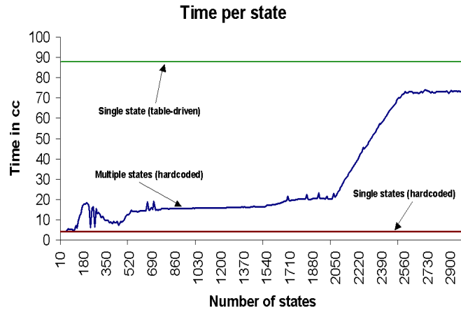
Figure 5. Hardcoded multiple state against single state implementation
