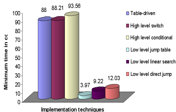
Figure 4. Average processing speed per implementation technique
