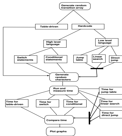
Figure 2. Process diagram indicating how the hardcoded implementation where compared to the table-driven implementation
