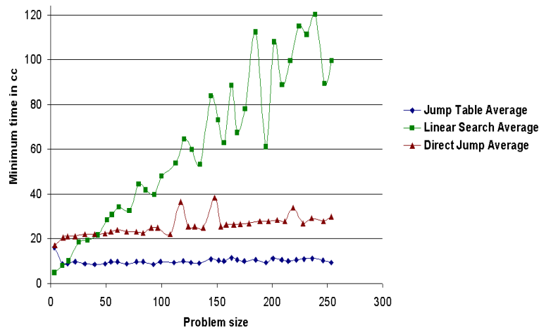
Figure 3. Performance based on rejecting symbols
